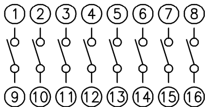
CIRCUIT DIAGRAM
